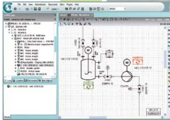
Maintenance information can be dynamically displayed in any desired document (e.g. P&ID)
